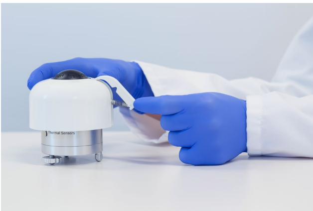
Figure 4 Pyranometer model SR30, with DP01 and sunscreen.
