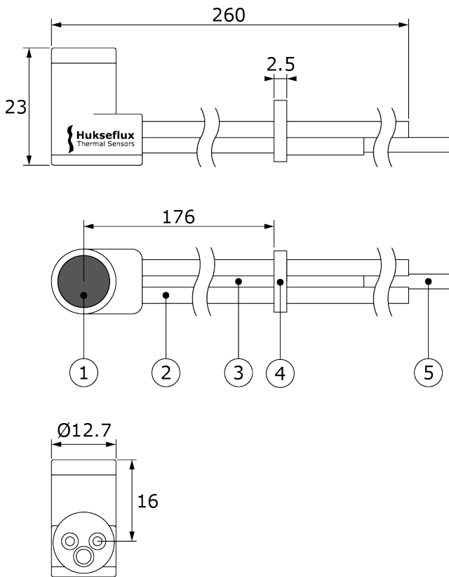
Figure 3 SBG04-100-02 standard model : (1) thermopile sensor with black coating, (2) water cooling tube, outer diameter tubes 3.2 \times 10^{-3} m, (3) sensor wire tube, (4) tube support ring, positioning stop for cone calorimeter, (5) cable, length 2 m. SBG04 is delivered with a practical protection cap for safe storage. All dimensions in \times 10^{-3} m.
