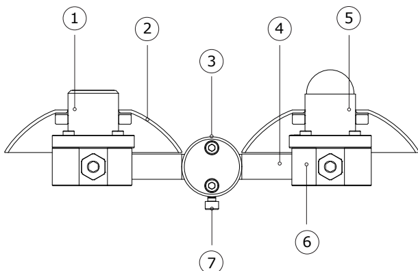
Figure 2 Overview of RA01: (1) upward facing pyrgeometer, (2) sun screens, (3,4,7) levelling assembly for x- and y-axis, (5) upward facing pyranometer, (6) instrument body.
