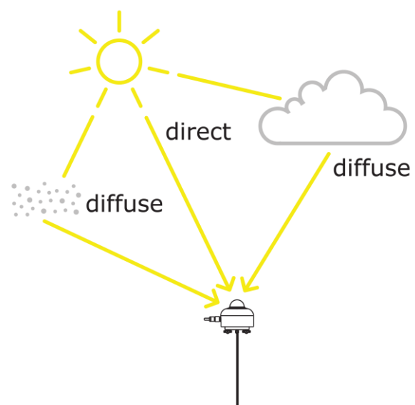
Figure 1 The global irradiance measured by the pyranometer includes direct sunlight and diffuse sunlight
