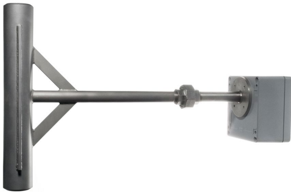
Figure 6 CBW01 heat flux sensor on a steam pipe. The sensor is located in the weld material at the crown of the tube. Typical use is in coal fired boilers and solar concentrators. Wiring is led away in the vertical tube to a connection box through the boiler insulation material. CBW01 is ASME certified.
