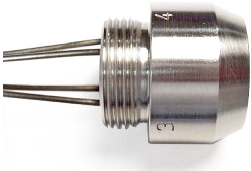
Figure 0.2 Example of a customer-specific RHF01 ring heat flux sensor with 4 x heat flux and temperature sensor
