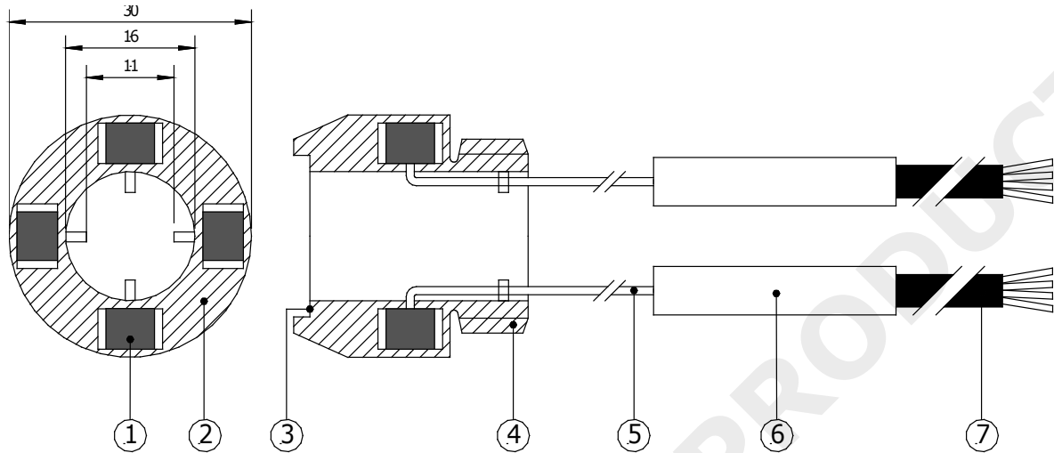
Figure 2.1 Example of RHF01 ring heat flux sensor with 4 x heat flux / temperature sensors (1), in a stainless steel body (2), with either a flat connection for welding- (3) or a threaded connection (4). High temperature cable (5) is usually extended with low temperature extension cable (7). Cooling must be provided by air, oil or water. RHF design is user-specific. Dimensions in the drawing serve as an example only. Dimensions are in \times 10^{-3} m.
