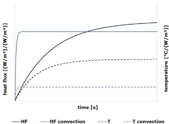
Figure 7 in situ sensor stability check. Comparison of responses to stepwise heating relative to reference curves. Normalised to heater power ( P ) and relative to the heat flux and the temperature just before heating. Solid graphs show heat flux, dotted graphs show temperature. The black HF and T signals are the reference curves at zero wind speed. The sensor is exposed to convection, which results in the blue responses: faster response times at lower heat flux and lower temperature rise.
