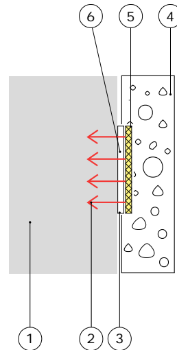
Figure 8 FHF02SC in a non-invasive core-temperature measurement. For measurement of the core temperature (1), the heater (5) is controlled to a setpoint of zero heat flux (2) measured by the heat flux sensor (3). At zero heat flux, the temperature of the core (1) and the temperature sensor (6) are equal. Insulation material (4) is attached to work at stable boundary conditions.
