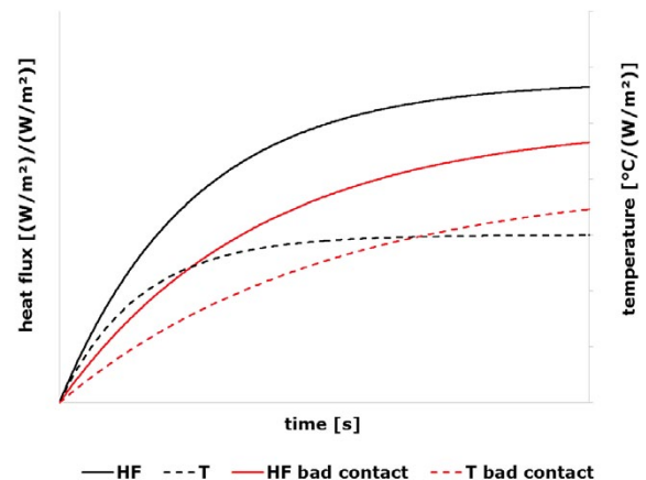
Figure 6 in situ sensor stability check. Comparison of responses to stepwise heating relative to reference curves. Normalised to heater power ( P ) and relative to the heat flux and the temperature just before heating. Solid graphs show heat flux, dotted graphs show temperature. The black HF and T signals are the reference curves at good thermal contact. The sensor loses thermal contact, which results in the red responses: slower response times, lower heat flux and higher temperature rise.
