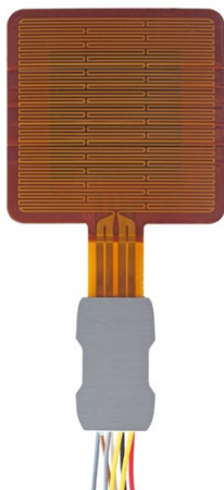
Figure 5 FHF02SC heat flux sensor's heater side
