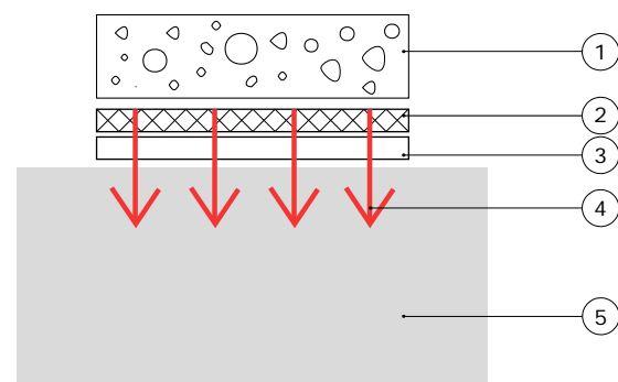
Figure 3 Calibration of FHF02SC; a typical stack used for calibration consists of a block of metal (mass > 1 kg), for example aluminium (5), the heat flux sensor (3), with heater (2) and an insulation foam (1). Under these conditions, heat losses through the insulation are negligible. Heat flux (4) flows from hot to cold.
