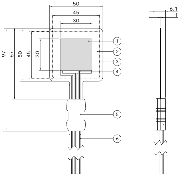
Figure 4 FHF02SC heat flux sensor: (1) sensing area with thermal spreader, (2) passive guard, (3) contour of the heater for self-test, (4) type T thermocouple, (5) strain relief block, (6) wires, standard length is 2 m. Dimensions in \times 10^{-3} m.
