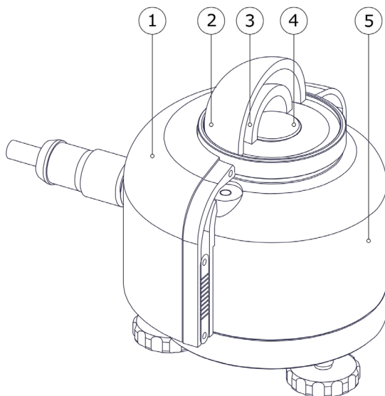
Figure 1 essential parts of a typical thermopile pyranometer: sunscreen (1), outer dome (2), inner dome (3), thermopile with sensor surface (4) and aluminium sensor body (5)
